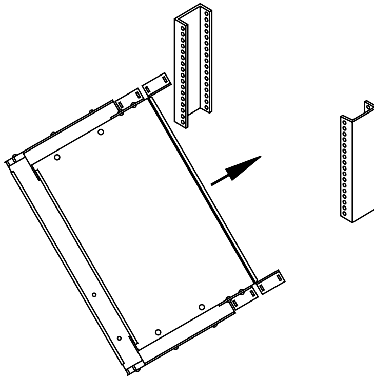
Figure 1. Lining up the shelf assembly on the rack.
