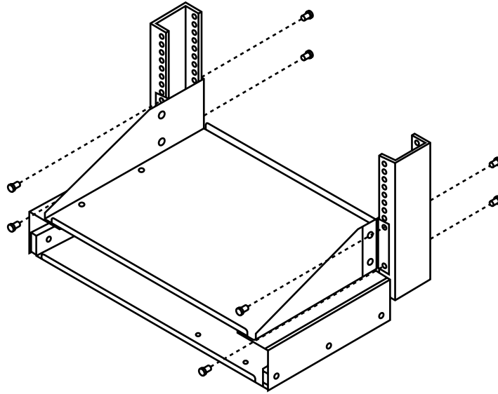
Figure 2. Attaching the assembly to the rack.
