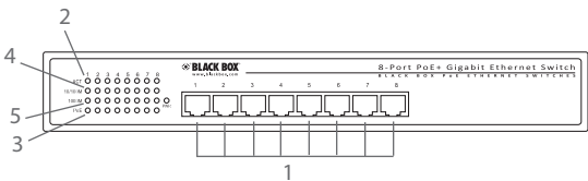
Figure 2-1. Front panel.
