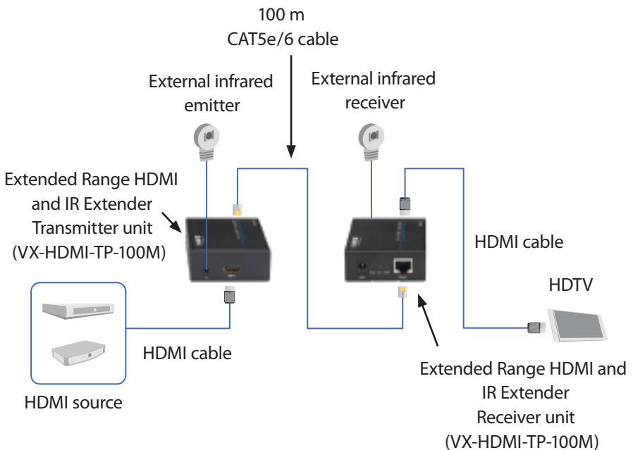
Figure 3-1. Connection diagram.
