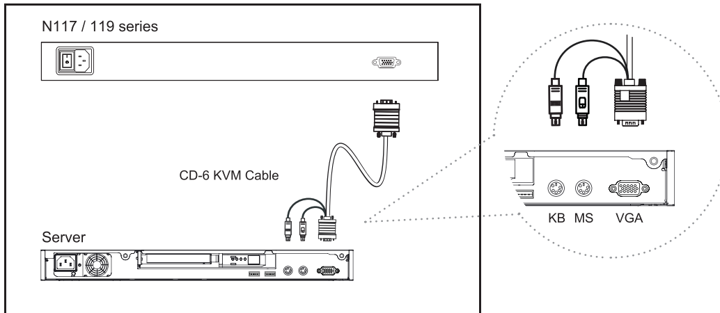
Figure 12. Example of connecting CD-6 3-in-1 PS/2 KVM cable to server via PS/2 interface
