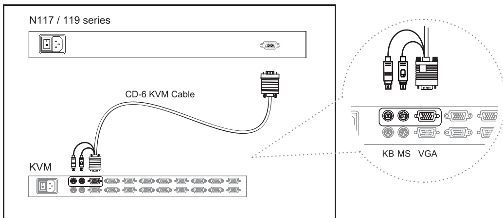
Figure 13. Example of connecting CD-6 3-in-1 PS/2 KVM cable to KVM via PS/2 interface
