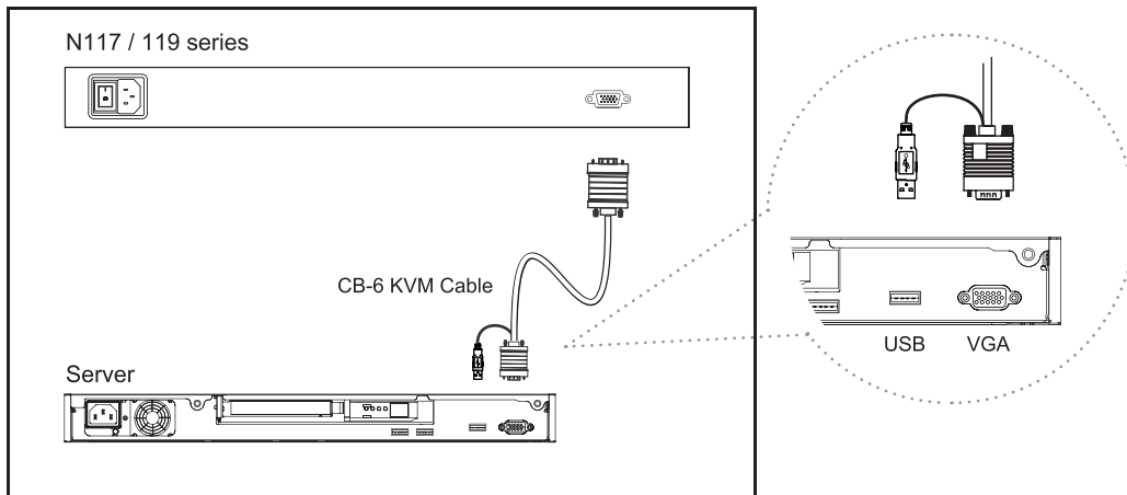
Figure 10. Example of connecting CB-6 2-in-1 USB KVM cable to server via USB interface
