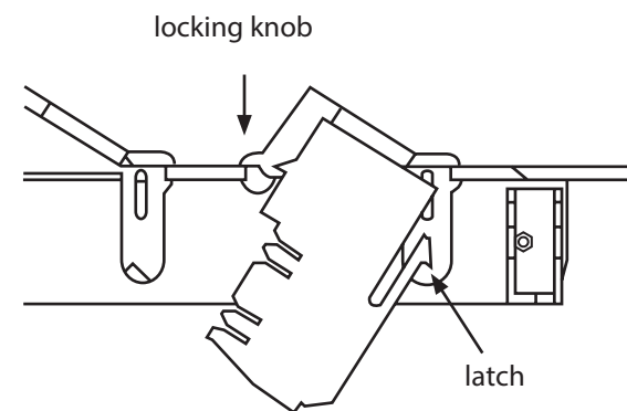
Figure 4. Loading the keystone jack or support fitting.
